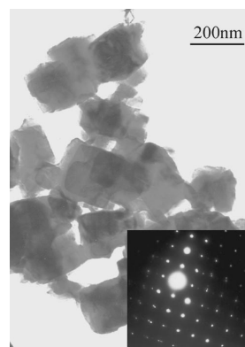
Figure 2. TEM image of the CaB 6 sample. Inset: Selected area electron diffraction pattern of CaB 6 .
