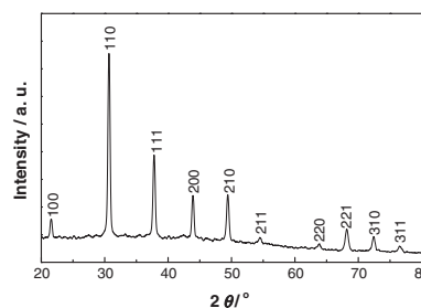
Figure 1. XRD patterns of the CaB 6 sample.
