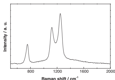
Figure 3. Raman spectra of the \text{CaB}_6 sample at room temperature.
