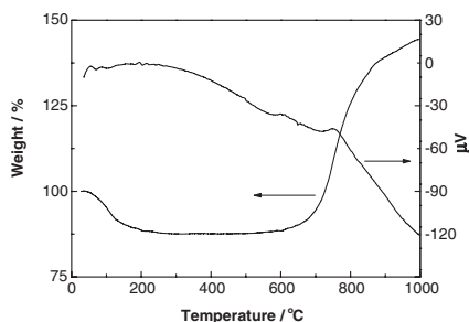
Figure 4. TGA and DTA curves for \text{CaB}_6 sample.
